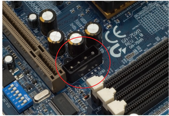
• Figure 10.21 Molex power on motherboard
