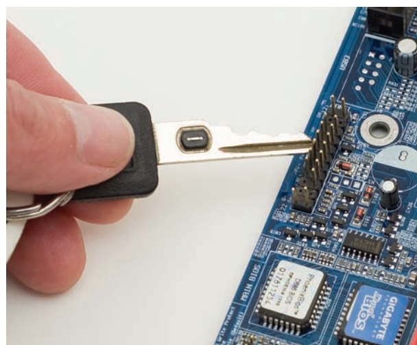
• Figure 10.30 Shorting the soft on/off jumpers
