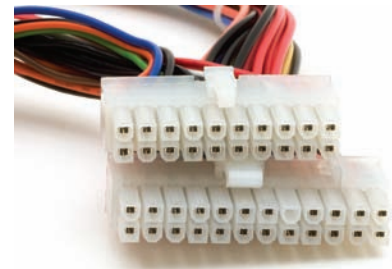
• Figure 10.22 20- and 24-pin connectors
