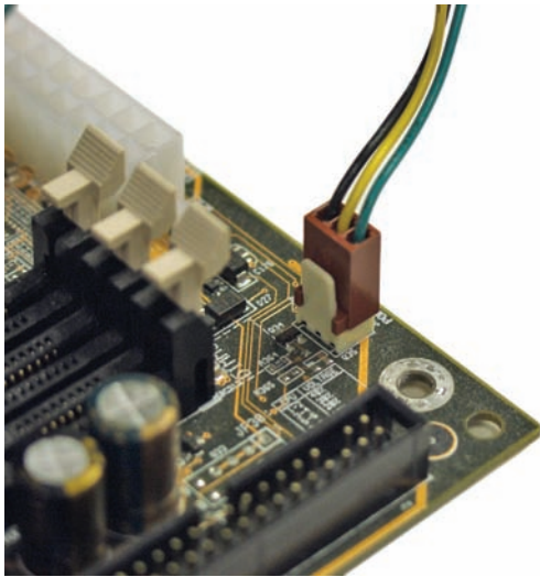
• Figure 10.32 3-wire fan sensor connector
