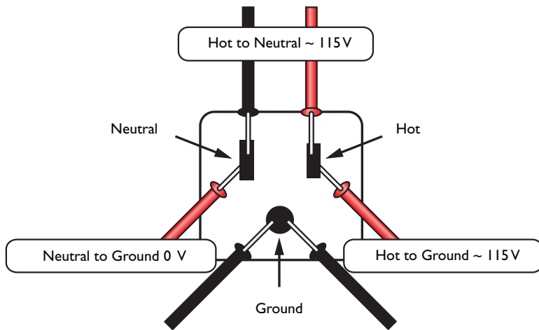
• Figure 10.4 Outlet voltages
