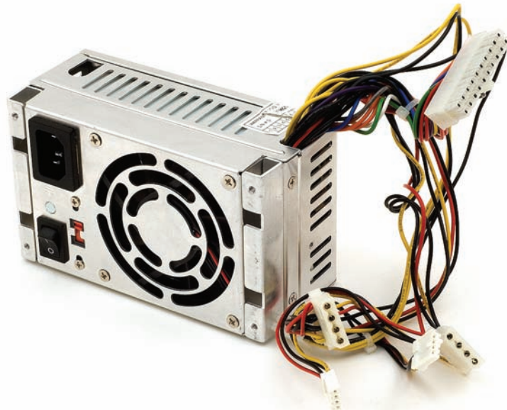
• Figure 10.25 SFX power supply
