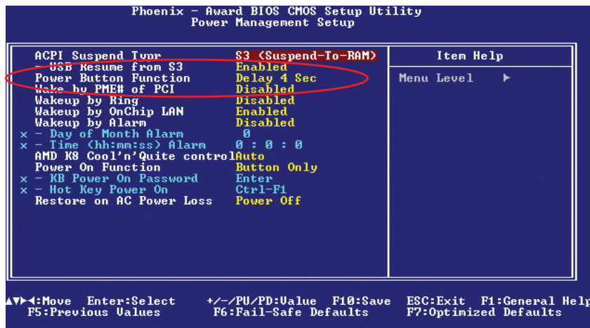
• Figure 10.19 Soft power setting in CMOS
