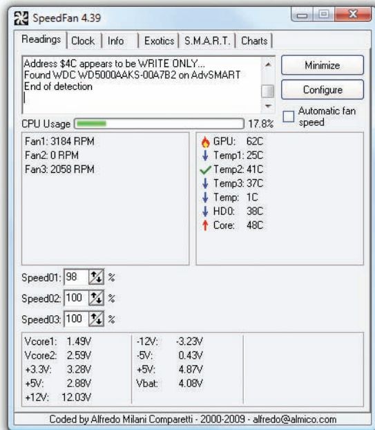
• Figure 10.37 SpeedFan
