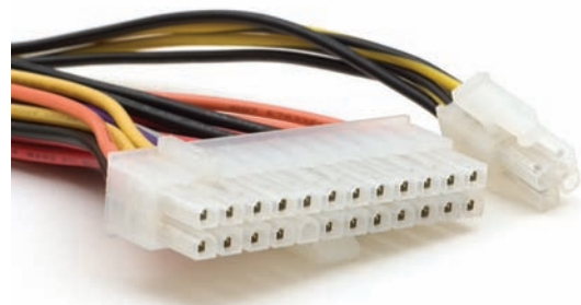
• Figure 10.13 Motherboard power connectors
