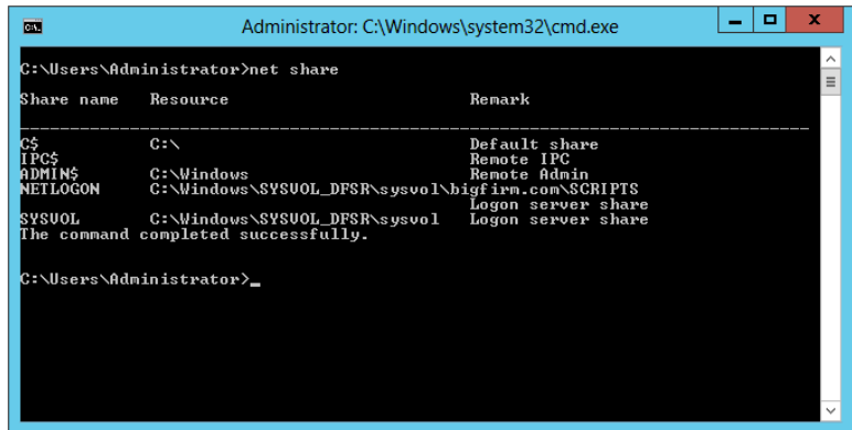
FIGURE 7.45 Final output of the net share command
