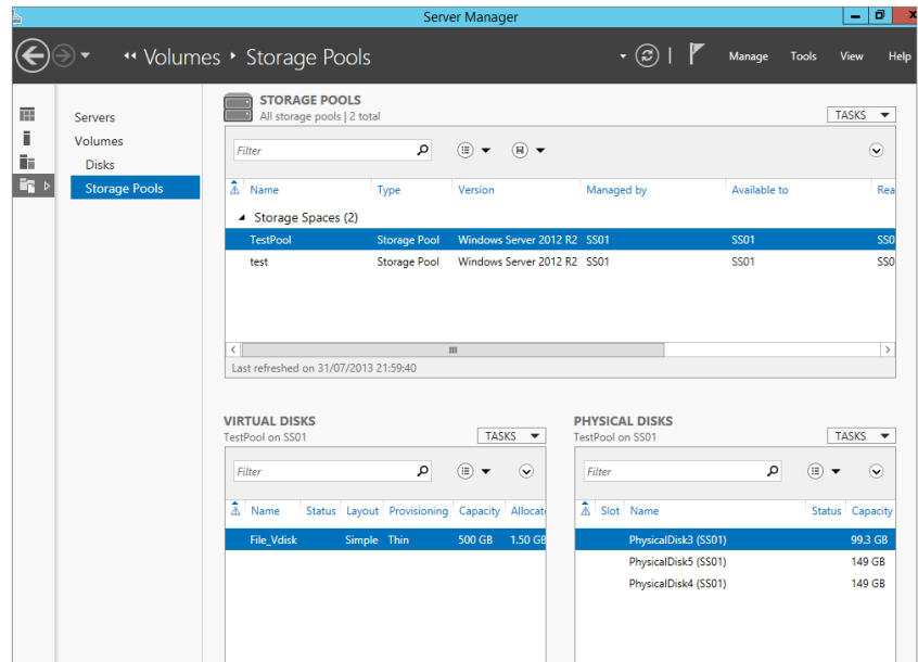
FIGURE 12.37 Storage Spaces UI with our newly created virtual disk
