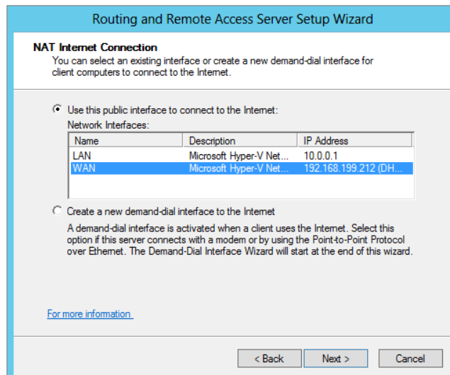
FIGURE 20.22 NAT Internet Connection screen—selecting the interface
