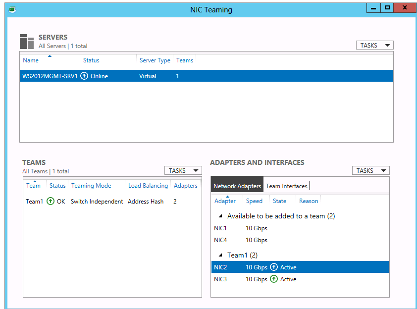
FIGURE 4.7 Newly created NIC team
