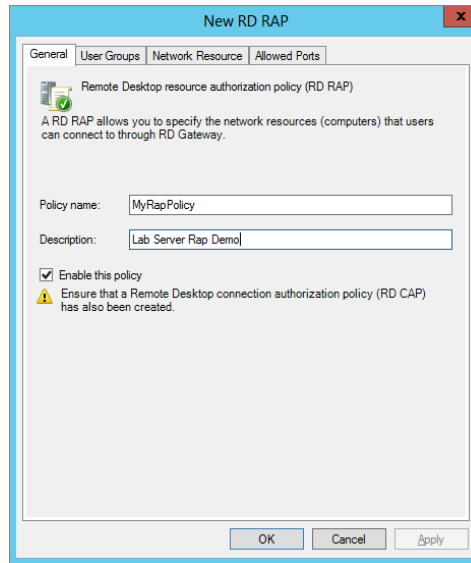
FIGURE 17.35 Add a policy name and description.
