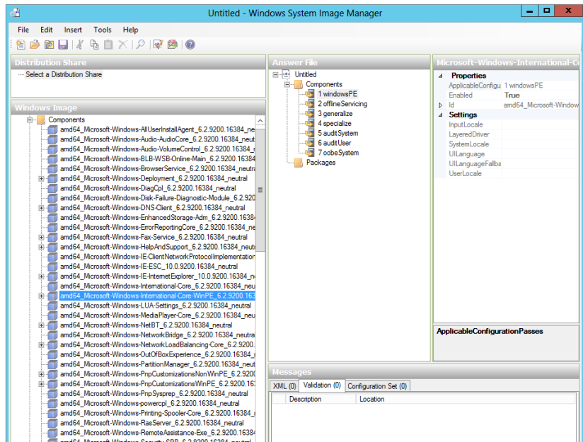
FIGURE 2.74 Select component to add to the answer file
