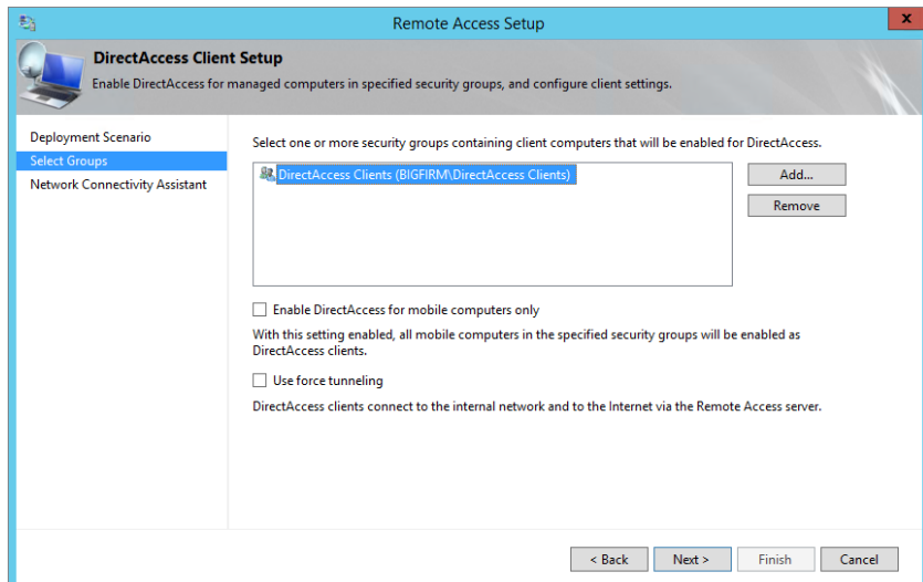
FIGURE 21.34 Selecting the DirectAccess Clients security group
