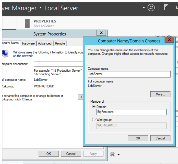
FIGURE 2.32 Domain membership change
