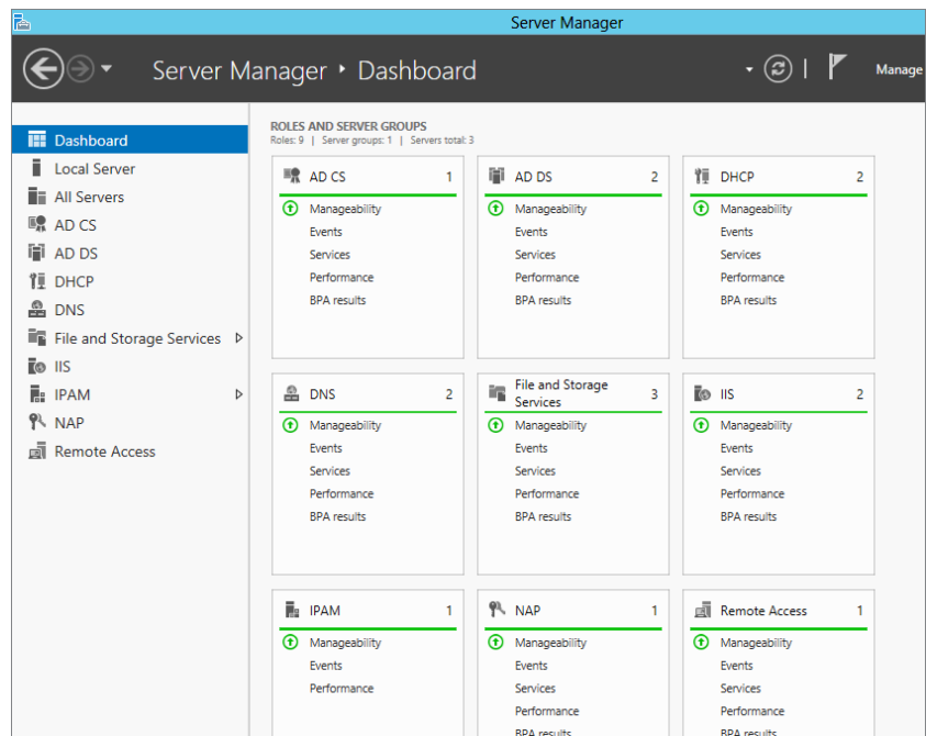
FIGURE 30.1 Monitoring multiple servers
