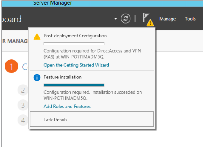
FIGURE 20.17 Post-deployment Configuration
