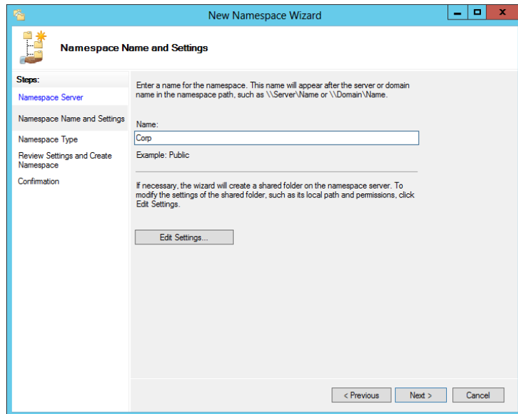
FIGURE 14.29 Namespace name
