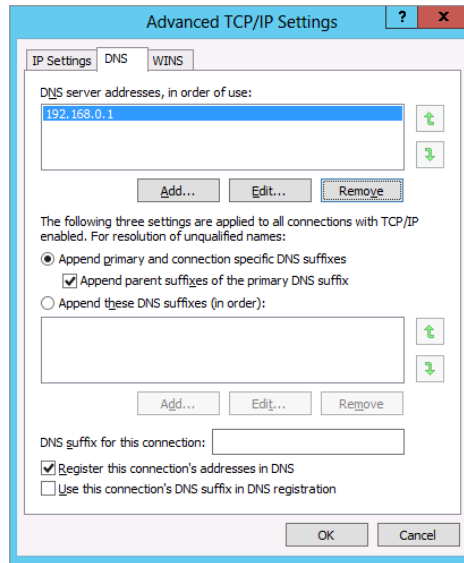
FIGURE 6.26 DNS tab
