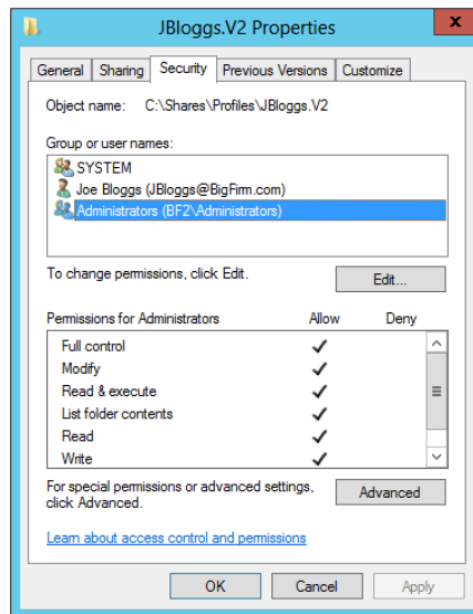
FIGURE 26.23 Administrators have access to roaming profile folders.
