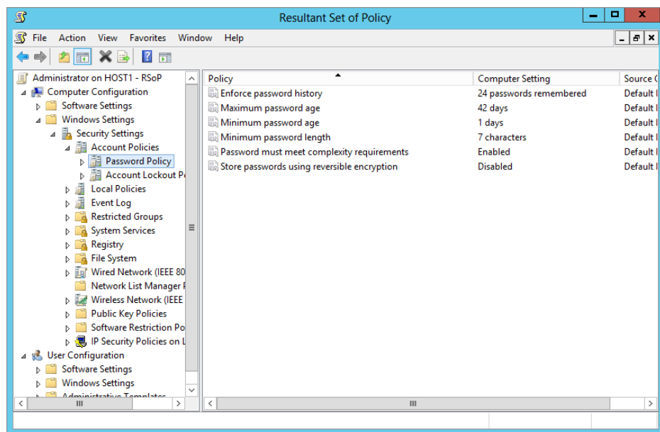
FIGURE 9.32 rsop.msc generates a real-time view of the policy settings that have been applied.
