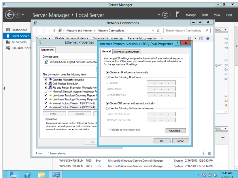
FIGURE 2.26 IPv4 properties
