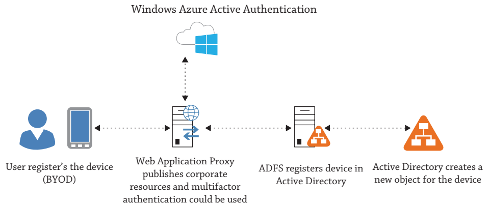
FIGURE 7.73 Workplace Join
