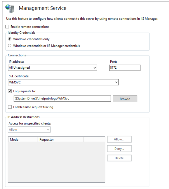
FIGURE 19.27 Management Service
