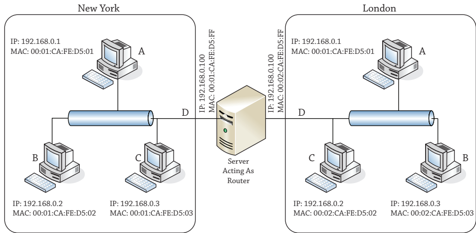
FIGURE 20.8 Sample network
