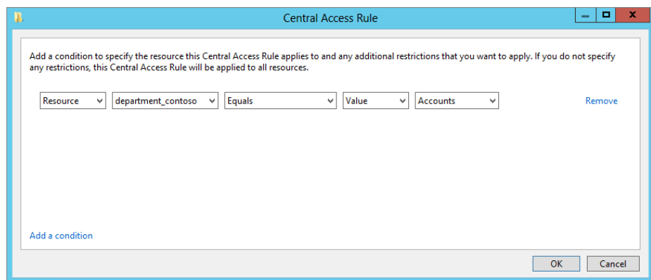
FIGURE 15.83 Resource targeting
