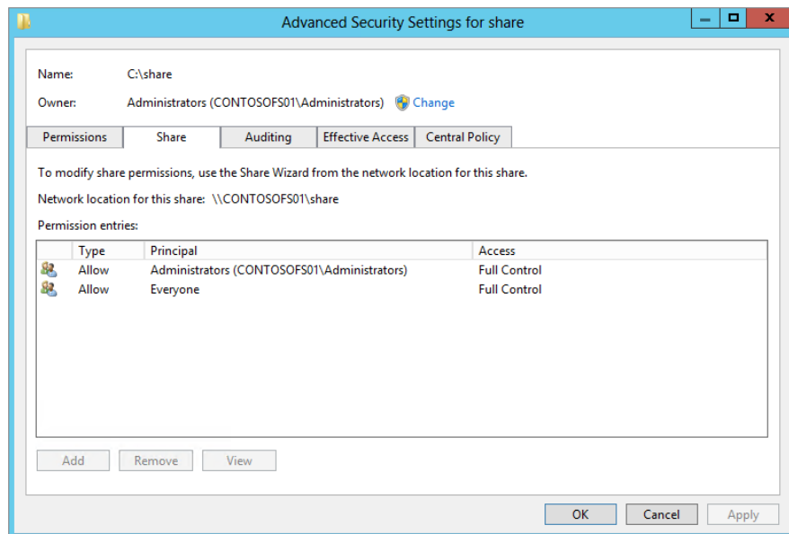
FIGURE 15.49 Share permissions
