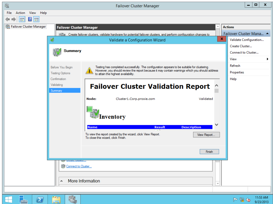
FIGURE 11.8 Validation Report
