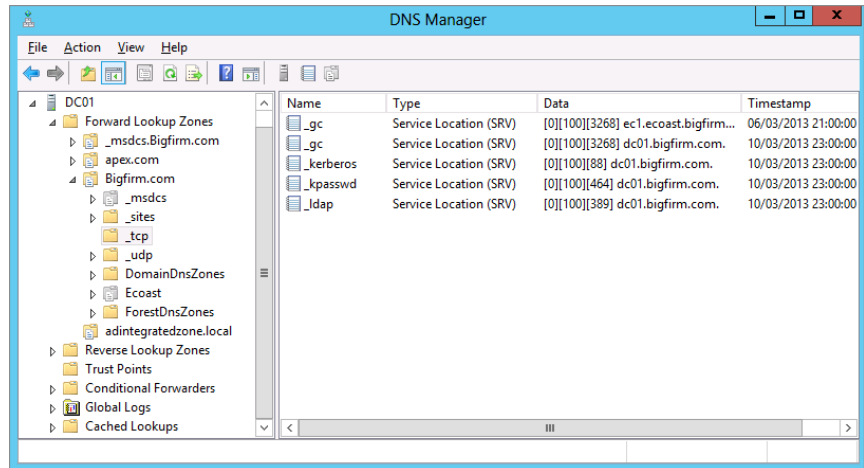
FIGURE 6.22 SRV record example
