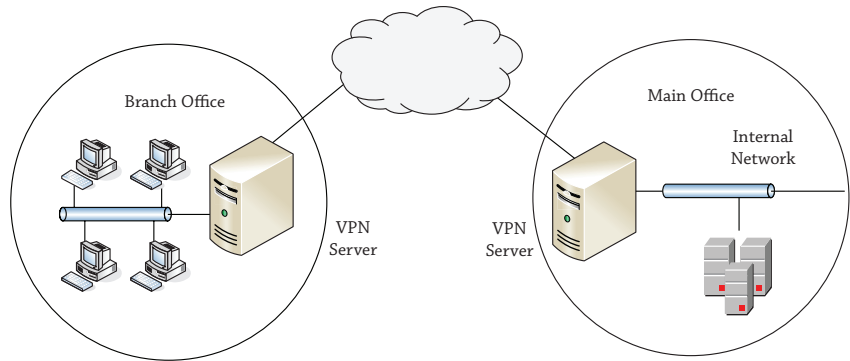
FIGURE 21.2 Gateway-to- gateway VPN
