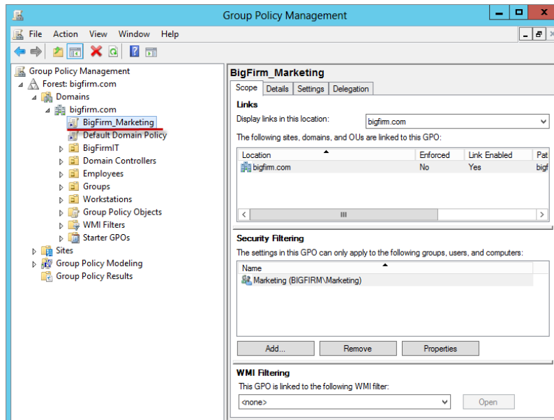
FIGURE 18.27 GPO applied to bigfirm.com
