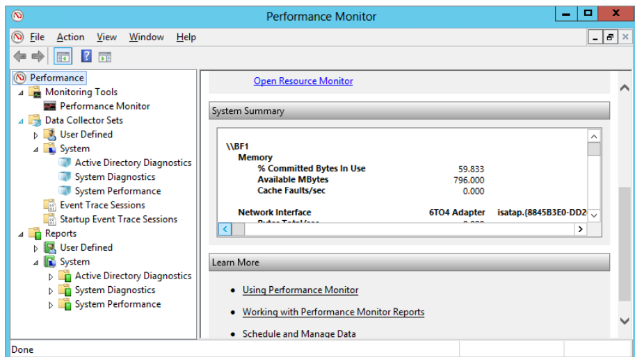
FIGURE 30.19 Performance Monitor
