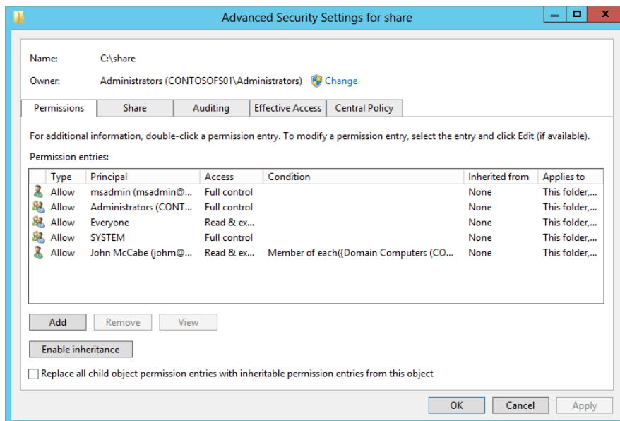
FIGURE 15.48 NTFS permissions
