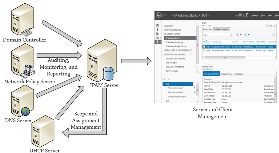
FIGURE 5.1 IPAM
