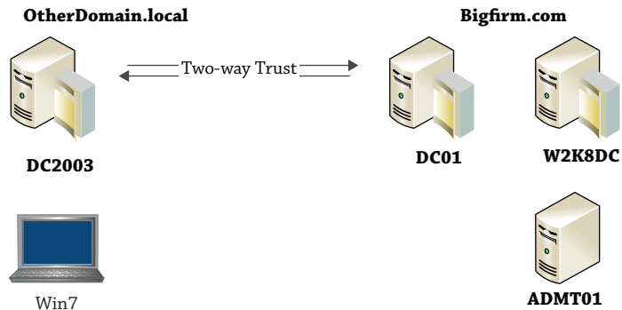
FIGURE 7.51 Migration scenario
